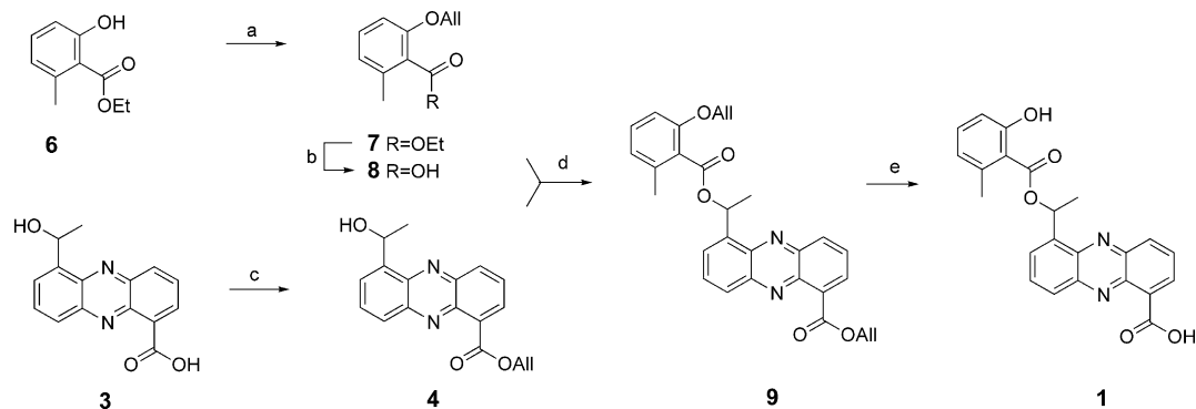
Scheme 2. Synthesis of saphenamycin; (a) All-Br, K 2 CO 3 , acetone, reflux 24 h (94%); (b) NaOH (s), EtOH/H 2 O, reflux, 30 h (98%); (c) All-Br, DIEA, CH 3 CN, rt 18 h (quant.); (d) (1) (COCl) 2 /DMF, CH 2 Cl 2 , 2 h; (2) DMAP, pyridine, room temp. 24 h. (64%); (e) Et 2 NH, Pd 0 (PPh 3 ) 4 (cat.), dioxane, rt 2.5 h. (88%). 88% of the R -isomer was obtained using optimized conditions as listed in this scheme. The racemic saphenamycin was prepared using non-optimized conditions that yielded 61%.
