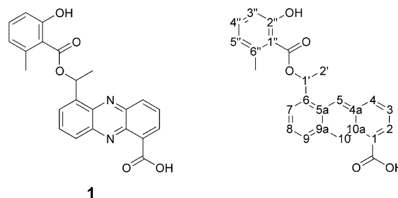
Figure 1. Structure and general atom numbering of saphenamycin ( 1 ).
