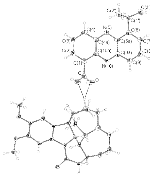
Figure 2. X-ray crystal structure of (–)-brucinium (–)-( R )-saphenate. Ellipsoids are 50% probability levels. 24 Hydrogen bonds between carboxylate of saphenic acid and ammonium salt of brucine are marked with thin lines and are 1.9 and 2.3 Å, respectively. Refinements were performed in SHELXL98 and the picture is created by ORTEP II.
