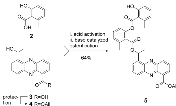
Scheme 1. Formation of 'double ester' byproduct when esterifying allyl saphenate ( 4 ) with excess 6-methylsalicylic acid ( 2 ).
